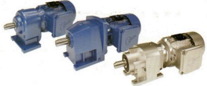
Inline Gear Unit
