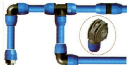
Aluminium Pipeline Fittings for Compressed Air - Application : Distribution of Compressed Air
